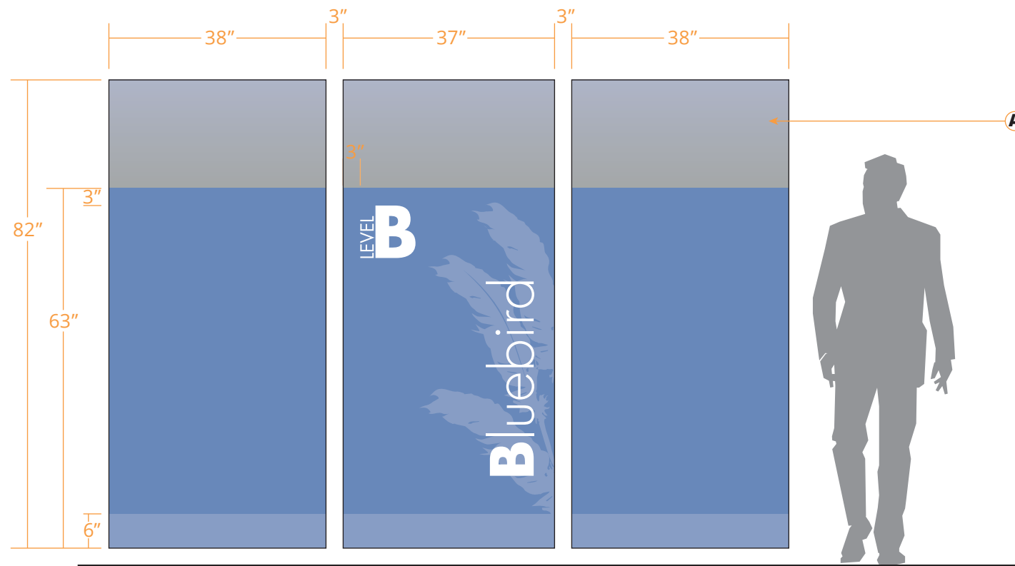
1 LEVEL B · ELEVATOR #1 scale: 1/2" = 1'-0"
