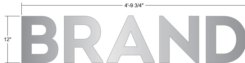
ID9 One (1) Set of Flat Cut Stainless Steel Letters Scale: 1" = 1'-0" Sq Ft: 4.81
