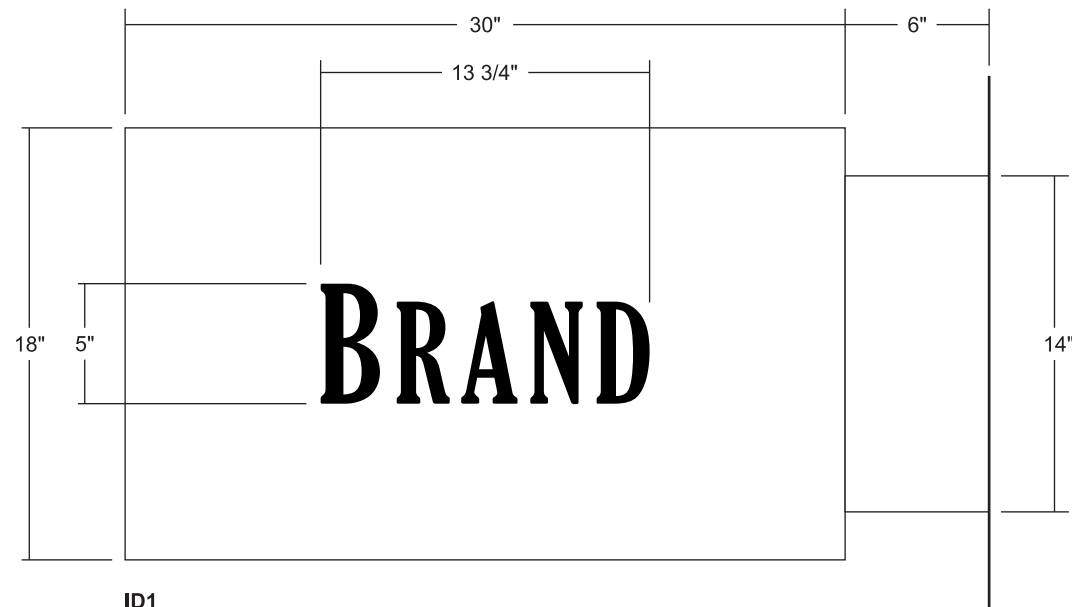
ID1 One (1) D/F Illuminated Blade Sign Scale: 1 1/2" = 1'-0" Sq Ft: 3.75
